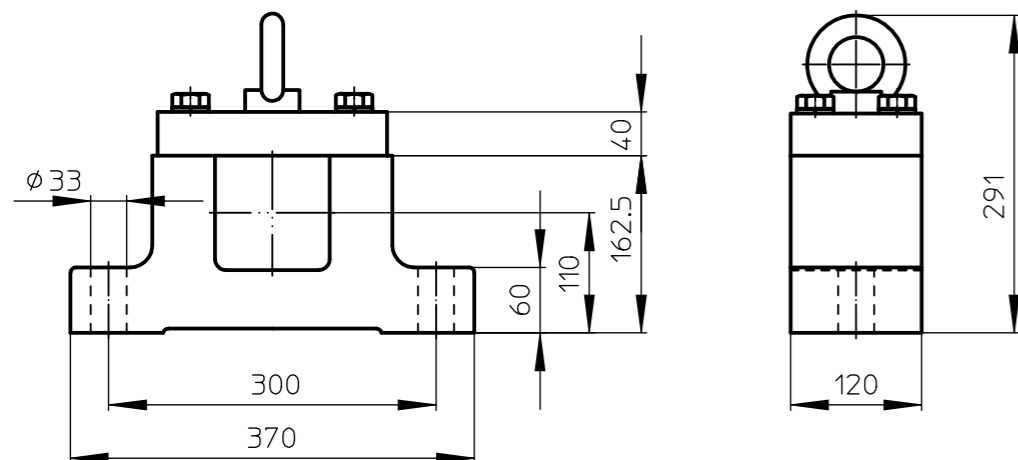
BRACKET AB130
