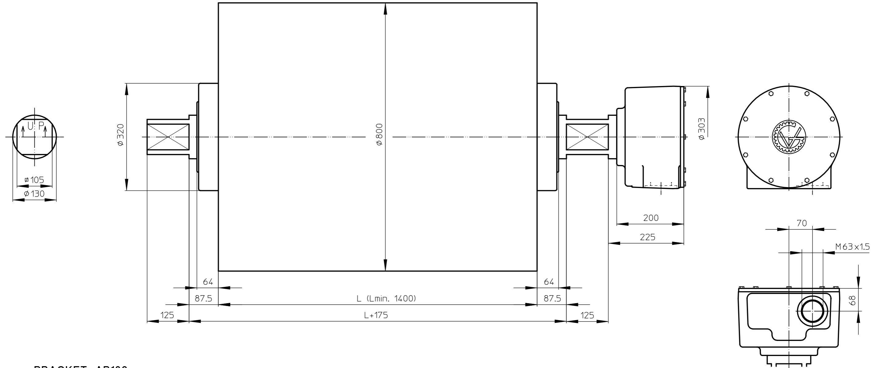
BRACKET AB130
